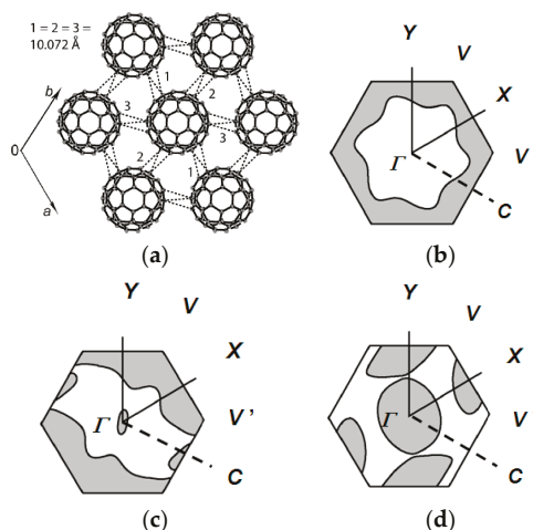
Figure 8. (a) View of the ab plane of fullerene Layer A in (TPC^0)(MDABCO^+)(C_{60}^{\bullet-}) at 300 K. The van der Waals C...C contacts shorter than 3.42 \text{ \AA} are shown by dashed lines. Numbers 1–3 indicate the r values; (b) The calculated Fermi surface of Layer A at 200 K, (c) that of Layers A at 160 K, and (d) that of Layer B at 160 K. (a) was reproduced from [12] and (b–d) were from [146].
