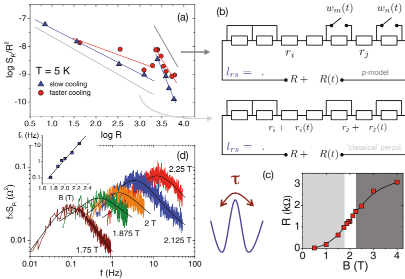
Figure 6. Percolation models in superconductors. (a) scaling of the normalized noise S_R/R^2 \propto R^{l_{rs}} of \kappa\text{-Cl}^* in a representation \log S_R/R^2 vs. \log R , where the slope reveals the power-law exponent l_{rs} , for data taken at T = 5 K and different magnetic fields up to 4 T as an implicate tuning parameter of the sample resistance (see (c)); (b) schematics of classical (bottom) and novel (top) percolation noise. In the former case ( l_{rs} = 0.9 ), the noise originates from the resistor elements, where the short-circuits represent superconducting subvolumes. The latter case of p -noise ( l_{rs} = 2.74 ) originates from switching elements controlled by random processes w_i(t) representing subvolumes with unstable superconductivity, after [72]. Reprinted with permission from [9]. Copyright (2011) John Wiley and Sons; (c) magnetoresistance R(B) at T = 5 K. Light and dark gray areas denote different percolation regimes characterized by the scaling exponent l_{rs} . In the white area, Lorentzian spectra are superimposed on the 1/f background noise (see (d)), where the inset shows the shift of the corner frequency f_c(B) . (a,d) reprinted with permission from [68]. Copyright (2009) by the American Physical Society.
