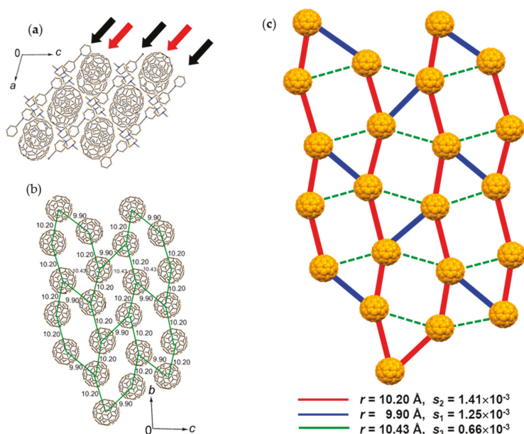
Figure 15. (a) Crystal structure of (PhCN 0 )(TMP + )(C 60 •− ) at 90 K viewed along the b axis. Black and red arrows indicate the layer of (PhCN 0 )(TMP + ) and (C 60 •− ), respectively; (b) View of the C 60 layer at 120 K showing the r \leq 10.20 Å by green lines; (c) Possible spin lattice geometry corresponding to (b) with overlap integrals; red line: s_2 = 1.41 \times 10^{-3} ( r = 10.20 Å), blue line: s_1 = 1.25 \times 10^{-3} ( r = 9.90 Å) and green line: s_3 = 0.66 \times 10^{-3} ( r = 10.43 Å) giving J_1:J_2:J_3 = 0.79:1:0.22 for the major C 60 orientation. Only one C 60 •− orientation is shown in (c). (a,b) were reproduced from [148].
