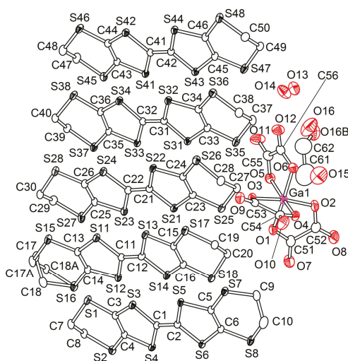
Figure 4. Asymmetric unit in 5 (50% level of thermal ellipsoids).
