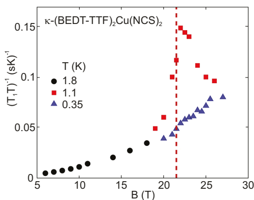
Figure 7. Field dependence of the spin-lattice relaxation rate, T_1^{-1} , divided by temperature of \kappa -(BEDT-TTF) _2 Cu(NCS) _2 . The data taken at 1.1 K exhibit an increase much beyond the normal-state value in the region where the FFLO phase occurs, whereas the effect is quenched at the lower temperature of 0.35 K. The dashed vertical line depicts the Pauli limit.
