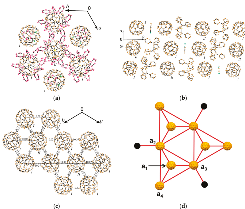
Figure 17. (a) Crystal structure of (\text{PhCl}_2^0)[(\text{Ph}_3\text{P})_3\text{Au}^+]_2(\text{C}_{60}^{\bullet-})(\text{C}_{60}) at 100 K viewed along the c axis (in the cationic supramolecule, C: red-violet, Cl: green, P: orange, Au: yellow). Only one of three orientations is shown for C 60 and PhCl 2 molecules. I: C 60 •− , II: C 60 0 ; (b) View along hexagonal C 60 layers and the diagonal of the ab plane. Black arrows indicate the (\text{PhCl}_2^0)[(\text{Ph}_3\text{P})_3\text{Au}^+]_2 supramolecule layer ( r_a = 10.37 Å, r_b \sim 13.92 Å); (c) View of the C 60 layer at 100 K for (\text{PhCl}_2^0)[(\text{Ph}_3\text{P})_3\text{Au}^+]_2(\text{C}_{60}^{\bullet-})(\text{C}_{60}) showing r in Å. Black dashed lines link C 60 centers. Four C 60 •− molecules (a 1 –a 4 ) form tetrahedral spin lattice with r = 10.37 Å and the a 1 molecule projects out of the a 2-4 plane by 3.03 Å; (d) Possible spin lattice geometry (red lines). Only one orientation of C 60 •− is shown. Black ball is C 60 •− . (a–c) were reproduced from [149].
