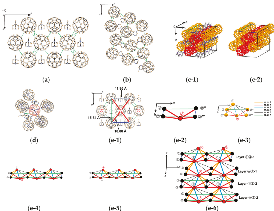
Figure 20. (a) View of crystal structure of (MDABCO^+)(C_{60}^{\bullet-}) along the a axis at 100 K; (b) View along the b axis at 100 K. The van der Waals contacts between fullerenes are shown in green dashed lines in (a,b); (c) C_{60}^{\bullet-} molecules stack along the b axis to form columns as shown with (c-1) or without MDABCO + (c-2, for simplicity). Yellow and red C_{60}^{\bullet-} columns are arranged alternately along the c axis to form a corrugated sheet in the bc plane; (d) Environment of one C_{60}^{\bullet-} radical anion (shown by red color) from eight neighboring C_{60}^{\bullet-} and five MDABCO + cations at 250 K. Center-to-center distances between red fullerene (A) and surrounding C_{60}^{\bullet-} (marked by numbers 1–3): A–1: 10.107, A–2: 10.081 and A–3: 10.008 Å. Van der Waals contacts between C_{60}^{\bullet-} and nitrogen atom of the MDABCO + cation are shown by green dashed lines. Only the major orientation of C_{60}^{\bullet-} is shown; (e) (e-1) Corrugated layer composed of molecules A and 2 at 250 K; (e-2) Geometry of a unit of possible spin lattice made of A and 2; (e-3) Schematic of bipyrimal spin lattice composed of molecules A, 1, and 2; (e-4) The unit shown by (e-3) forms 2D layer by sharing an edge. Only the ribbon extending along the c axis is shown; (e-5) The other unit of bipyrimal spin lattice composed of 1, A, and 3 forms equivalent 2D layer; (e-6) The model geometry of the possible spin lattice obtained by sharing apexes of the layer in (e-4,e-5) along the a axis to form a 3D distorted bipyrimal spin lattice (a,b,d), (e-1) from [147]).
