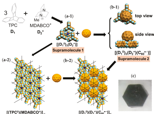
Figure 4. The formation of two-dimensional (2D) C_{60}^{\bullet-} layer (Layer A) on the polycationic template of [(TPC^0)(MDABCO^+)]_\infty : Three TPC ( D_1 ) and one MDABCO + ( D_2^+ ) molecules form the first supramolecular unit ((a-1): Supramolecule 1 [(D_1^0)_3(D_2^+)] ), and a C_{60}^{\bullet-} molecule fits into the concave to form the second supramolecular unit ((b-1): Supramolecule 2 [(D_1^0)_3(D_2^+)](C_{60}^{\bullet-}) ). They assemble to form a 2D layer (Layer A) of hexagonal packing of C_{60}^{\bullet-} ((b-2): [(TPC^0)(MDABCO^+)(C_{60}^{\bullet-})]_\infty ). In another view, the 2D arrangement of the first supramolecular units (a-2), where N atoms of MDABCO agglomerate at the crossing points of lines, works as a cationic template to arrange C_{60}^{\bullet-} molecules at the crossing points to form hexagonal layer of C_{60}^{\bullet-} (Layer A) (b-2). (N: blue, H: pale blue, C: yellow). The thin lines in (a-2,b-2) are a guide to the eye. (c) Single crystal showing the ab face.
