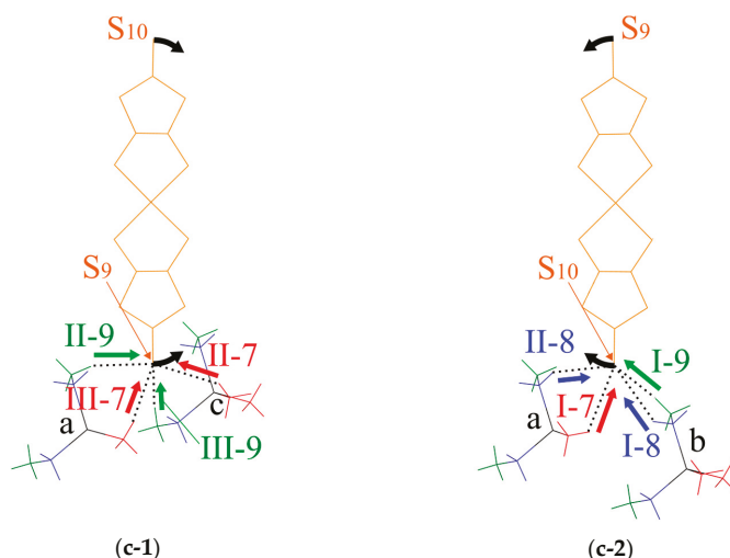
Figure 9. Schematic illustration of the short S...H-C contacts. (a) Oblique view. (b) End-on projections of the dimer arrangement. (c) Views along the vector connecting the two Pd atoms in the dimer, (c-1) shows the short S...H-C contacts between the S 9 atom in the lower Pd(dmit) 2 molecule in (b) and cations a and c , (c-2) shows the S...H-C short contacts between the S 10 atom in the upper Pd(dmit) 2 molecule in (b) and cations a and b ; black arrows indicate the direction of the arch-shaped distortion with a positive \Phi value. The red, green and blue arrows indicate the directions of repulsive S...H-C7, S...H-C8, and S...H-C9 interactions, respectively.
