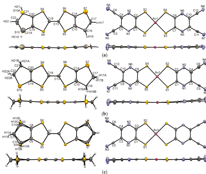
Figure 1. ORTEP and atomic numbering schemes (top and side views) of (a) \alpha -DT-TTF donor molecule and acceptor [Au(dcdmp)_2] molecule in the crystal structure of 1; and (b,c) BET-TTF donor molecule and acceptor [Au(dcdmp)_2] molecule in the crystal structure of 2: (b) structure M (2M) and (c) structure T (2T). Thermal ellipsoids drawn at 70% probability level.
