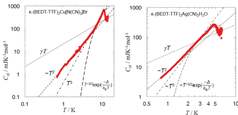
Figure 9. Temperature dependence of the electronic heat capacity determined as the difference of the 0-T data and the normal state data obtained under magnetic fields higher than H_{c2} for (a) \kappa -(BEDT-TTF) _2 Cu[N(CN) _2 ]Br and (b) \kappa -(BEDT-TTF) _2 Ag(CN) _2 H _2 O below the transition temperatures. (Ref. [60].) The lines and the curve shown in the figure denote T linear, T^2 , T^3 , and T^{-3/2}\exp(-\Delta/k_B T) temperature dependence.
