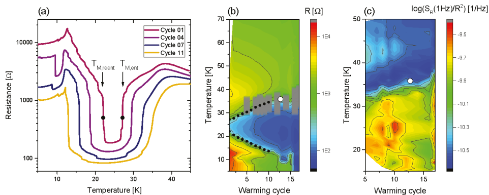
Figure 12. Resistance and noise measurements at the Mott transition in partially-deuterated \kappa\text{--[}(\text{H}_8\text{-ET})_{1-x}(\text{D}_8\text{-ET})_x\text{]}_2\text{Cu[N(CN)}_2\text{]Br} with x = 0.75 . (a) resistance measurements of some selected warming cycles generated by using different thermal relaxation protocols described in the text. The black points mark the temperatures of the entrance and re-entrance half-maximum resistance jump, indicating the crossing of the Mott transition line; (b) contour plot of the resistance vs. temperature and warming cycle. The grey area marks the region where the DDH model shows strong deviations; the white circle indicates the critical point; (c) contour plot of the normalized resistance noise PSD taken at 1 Hz in dependence of temperature and warming cycle (note different scales).
