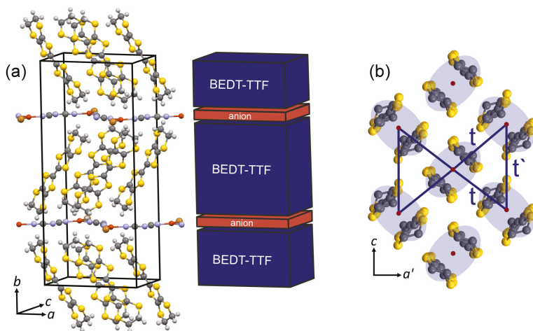
Figure 1. (a) crystal structure (left) of \kappa -(BEDT-TTF) _2\text{Cu}[\text{N}(\text{CN})_2]\text{Z} with \text{Z} = \text{Br}, \text{Cl} , which can be simply viewed as alternating blocks (right) of conducting layers with the donor ET and polymeric chain-forming acceptor \text{Cu}[\text{N}(\text{CN})_2]\text{Z} molecules, respectively. The box represents the unit cell hosting four formula units; (b) spatial arrangement of the ET molecules in the \kappa -phase viewed along the long axis of the molecules. Two ET molecules form a dimer (shaded ellipse), whereas two dimers are arranged almost orthogonal to each other. Considering the dimers as the basic structural units, the conduction band is effectively half-filled and the charge carriers reside on a triangular lattice with two transfer integrals t and t' .
