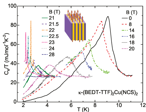
Figure 3. Electronic part of the specific heat of \kappa -(BEDT-TTF) _2 Cu(NCS) _2 , vs. temperature in parallel magnetic fields (inset) up to 28 T.
