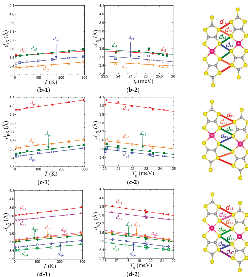
Figure 7. Temperature dependence of intermolecular S···S distances associated with T_B (a-1), T_r (b-1), T_p (c-1), and T_q (d-1) in the EtMe 3 Sb salt. Relationships between the S···S distances and intermolecular transfer integrals, T_B (a-2), T_r (b-2), T_p (c-2), and T_q (d-2) in the EtMe 3 Sb salt.
