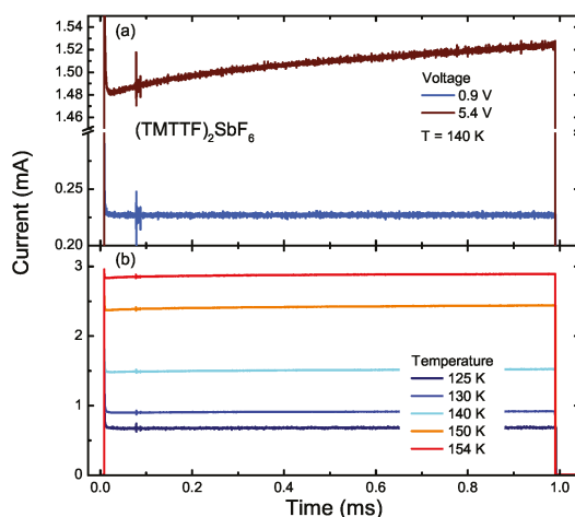
Figure 7. (a) Response of the current in (\text{TMTTF})_2\text{SbF}_6 , when 1\text{ ms} pulses of two different voltages are applied at T = 140\text{ K} ; (b) Current response plotted for various temperatures below T_{\text{CO}} .
