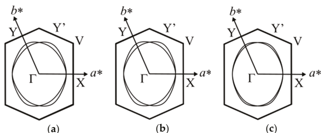
Figure 4. Fermi surface of the EtMe 3 Sb salt calculated by the extended Hückel and tight binding methods at 5 K (a), 101 K (b), and 295 K (c). The C-centered monoclinic cell is reduced to the primitive one as a_p = (a + b)/2 , b_p = b , c_p = c .
