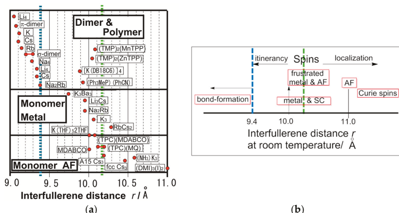
Figure 3. (a,b) Bond formation (dimer and polymer), monomer metal, and monomer AF regions of C_{60}^{n-} with the center-to-center interfullerene distance r at RT except [K(DB18C6)]_4(C_{60})_5 \cdot 12THF (225 K indicated as [K(DB18C6)]_4 ), \{(TMP^+)_2M^{II}TPP\}(C_{60}^{\bullet-})_2(PhCN)_2(PhCl_2)_2 (270 K indicated as (TMP)_2(MnTPP) and 250 K indicated as (TMP)_2(ZnTPP) , K(C_{60}^{\bullet-})(THF)_5 \cdot 2THF (260 K indicated as K(THF)_5 \cdot 2THF ) and (MDABCO)(C_{60}^{\bullet-}) (250 K indicated as MDABCO ). Cation or donor species are shown in boxes and Figure 2a. Li_4 and Cs are plotted twice according to different interfullerene distances in the 2D polymer and in different phases (polymer or dimer), respectively. K(THF)_5 \cdot 2THF and (TPC)(MDABCO) are located on the borderline between monomer metal and monomer AF. Blue dotted line and green one indicate r = 9.4 Å and van der Waals diameter of C_{60} (10.18 Å), respectively.
