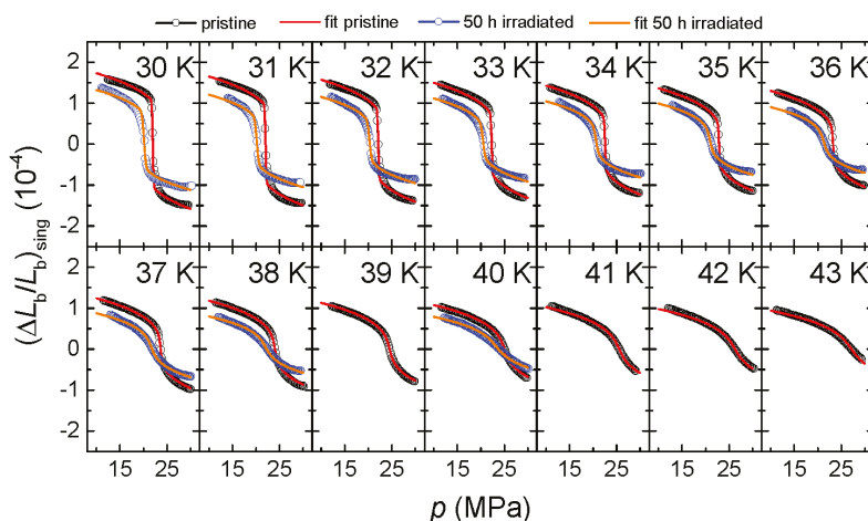
Figure 4. Singular part of the relative length change of \kappa -(BEDT-TTF) 2 Cu[N(CN) 2 ]Cl along the out-of-plane b axis, (\Delta L_b/L_b)_{\text{sing}} , (open symbols) as a function of pressure p at various temperatures 30 \text{ K} \leq T \leq 43 \text{ K} , together with a fit (straight lines) based on the mean-field solution, given by Equation (1). Black open symbols and red straight lines represent results on a pristine sample of batch #AF063, which were published in Ref. [25]. Blue open symbols and orange lines represent results on a crystal of batch #AF063 which was exposed to X-ray for 50 h.
