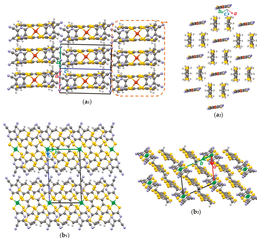
Figure 6. Crystal structure of compound 5 (a) and compound 6 (b): (a 1 ) view along a - b ; (a 2 ) partial view along the long axis of the molecules of neighbouring columns in the same layer, with the alternating dianions and BET-TTF dimers; (b 1 ) view along the stacking axis; (b 2 ) partial view of the layers in the ab plane.
