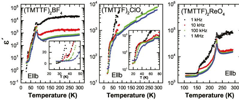
Figure 18. Temperature dependence of the real part of the dielectric permittivity \epsilon'(T) measured with E \parallel b' for (\text{TMTTF})_2\text{X} with \text{X} = \text{BF}_4 , \text{ClO}_4 and \text{ReO}_4 at different frequencies as indicated. The insets emphasize the changes close T_{\text{AO}} and below.
