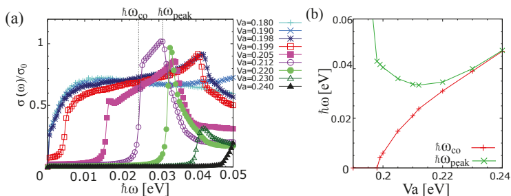
Figure 2. The optical conductivities divided by the universal conductivity \sigma_0 = \pi e^2 / 2h [38] for V_a = 0.180, 0.190, 0.198, 0.199, 0.205, 0.212, 0.220, 0.230, 0.240 (a). \omega_{\text{CO}} and \omega_{\text{peak}} for V_a = V_a^{c2} = 0.212 are shown in (a). V_a -dependences of \omega_{\text{CO}} and \omega_{\text{peak}} are shown in (b). A characteristic peak structure is found near the CO transition in the extended Hubbard model describing the organic Dirac electron system \alpha -(BEDT-TTF) _2 I _3 .
