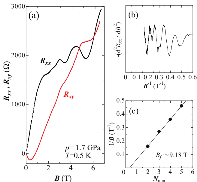
Figure 10. (a) Magnetic field dependence of R_{xx} , R_{xy} , and (b) SdH oscillation ( -d^2 R_{xx}/dB^2 ) under the pressure of 1.7 GPa at 0.5 K; (c) value of B^{-1} for the SdH oscillation minima. In the Dirac electron systems, the linear extrapolation of the data to B^{-1} = 0 should be 1/2 . For normal electrons, on the other hand, it is shifted to 0.
