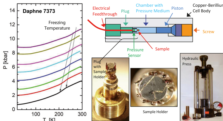
Figure 8. Left panel: Pressure loss of Daphne 7373 oil during cooling; the arrows mark the temperature range of freezing. The data were recorded in a Copper-Beryllium cell by four-point resistance measurement of an InSb pressure sensor. Right panel: Sketch of the actual pressure cell used and photos of the sample holder, and the hydraulic press.
