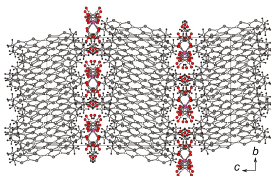
Figure 5. Projection of the structure 5 along a.
