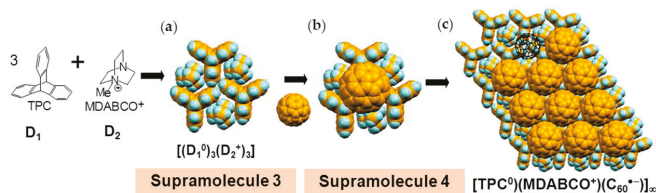
Figure 7. Formation of a 2D C_{60}^{\bullet-} layer (layer B) on the polycationic template of [(TPC^0)(MDABCO^+)]_\infty : (a) Three TPC^0 ( D_1 ) and three MDABCO^+ ( D_2^+ ) molecules form Supramolecule 3 [(D_1^0)_3(D_2^+)_3] ; (b) A C_{60}^{\bullet-} molecule fits into the concave to form Supramolecule 4 [(D_1^0)_3(D_2^+)_3] C_{60}^{\bullet-} ; (c) 2D layer (Layer B) of hexagonal packing of C_{60}^{\bullet-} by assembly of Supramolecule 4 .
