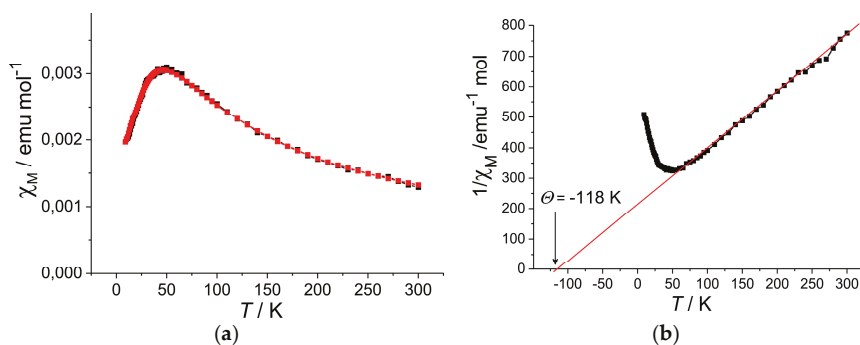
Figure 21. Temperature dependence of molar magnetic susceptibility \chi_M (a) and 1/\chi_M (b) of (MDABCO) + ( C_{60}^{\bullet-} ) after correction of Curie impurity. Red curve in (a) is the fit by the Heisenberg model for square 2D AF coupling of spins with J/k_B = -25.3 K. Red line in (b) is the Curie-Weiss fit with \Theta_{CW} = -118 K [147].
