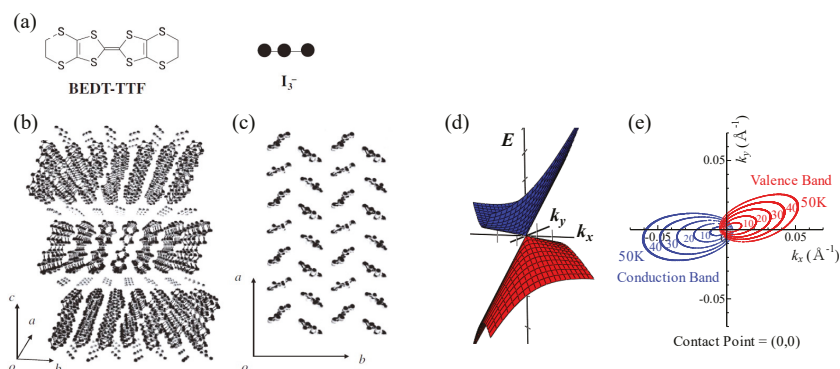
Figure 1. (a) BEDT-TTF molecule and I_3^- anion, crystal structure of \alpha -(BEDT-TTF) _2I_3 viewed from (b) a -axis and (c) c -axis, (d) band structure, and (e) energy contours near a Dirac point. Note that we take the origin to the position of the Dirac point.
