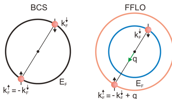
Figure 1. Color online. From Wosnitza [35] On the left, the traditional BCS Cooper pair is represented. On the right, the energy of the up and down electrons have been shifted by the magnetic field. A momentum \mathbf{q} can be added to one of the electrons to create a zero momentum center of mass Cooper pair. In the diagram, the initial momentum of the electrons is isotropic. In real material, the shape of the Fermi surface could create more complex diagrams.
