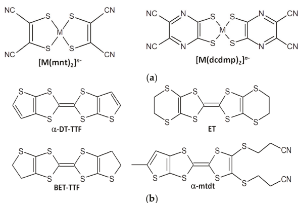
Scheme 1. Molecular diagram of transition metal bisdithiolene complexes (a) and of TTF type donors (b).
