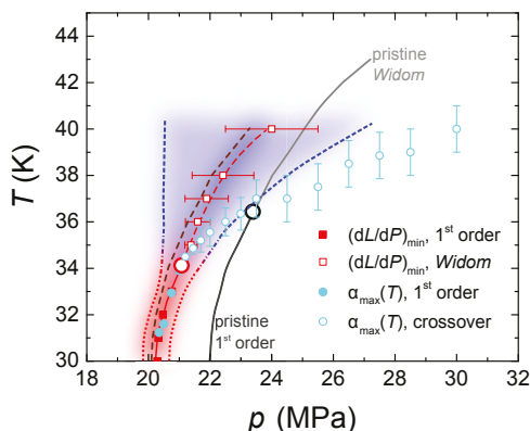
Figure 3. Experimentally determined temperature-pressure phase diagram of \kappa -(BEDT-TTF) _2 Cu[N(CN) _2 ]Cl (batch #AF063) after exposure to X-ray for 50 h. Red full squares correspond to the first-order Mott transition line extracted from the inflection point of \Delta L_b(p)/L_b . Cyan full circles correspond to the first-order transition line extracted from temperature-dependent measurements. The latter data points were determined by the position of the maximum \alpha_{max} of the thermal expansion coefficient \alpha_b(T) = L_b^{-1} dL_b/dT for p < p_c . Red open symbols correspond to the Widom line. Open cyan symbols correspond to a crossover line, determined by the position of \alpha_{max} for p > p_c . Red- and blue-shaded areas delimited by the broken lines in the same color code indicate the experimentally determined width of the features along the b axis and can be assigned to the disorder-related (red) and the criticality-related (blue) crossover regimes, respectively. The broken lines represent, within the error margins, the full width at half maximum of the peaks in dL/dP . The brown dashed line corresponds to the p_c(T) curve extracted from a fit of the data, presented in Figure 1 to the mean-field model of Equation (1) (see text for details). The first-order transition line (dark grey line), the Widom line (light grey line) and the critical endpoint (black open circle) for a pristine crystal of batch #AF063 [25] are given for comparison.
