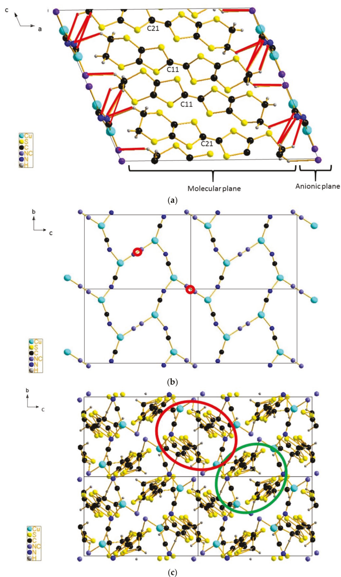
Figure 3. (a) (color online) Structure of \kappa -ET-Cu at 300 K viewed along the b -axis. For clarity purpose, only the most probable staggered C_2H_4 group configurations are represented. In the molecular layer, the first number of the atom labels (1 or 2) refers to the two different types of molecules and are indicated for the C11 atoms only. The hydrogen bonds (red lines) of the ethylene groups (S conformation) with the N and disordered N/C atoms in the anionic plane are also shown; (b) View of the anionic plane parallel to the ( b , c ) plane: the disordered C–N groups, which are located on the inversion centers (red circles), are colored in violet; (c) View of the anionic ( b , c ) plane and the molecular layer below showing Dimer 1 (green) and Dimer 2 (red).
