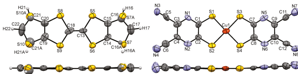
Figure 3. ORTEP and atomic numbering schemes (top and side views) of donor molecules and acceptor [Cu(dcdmp) 2 ] − in the crystal structure of \alpha -DT-TTF[Cu(dcdmp) 2 ] ( 3 ), with thermal ellipsoids drawn at 70% probability level.
