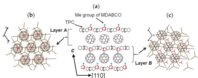
Figure 6. Crystal structure of (TPC 0 )(MDABCO + )(C 60 •− ) at 160 K: The (TPC 0 )(MDABCO + ) layer and C 60 •− layer stack along the c axis with the sequence of the Layer A of C 60 •− /(TPC 0 )(MDABCO + ) layer/Layer B of C 60 •− . (a) C 60 •− molecules in Layer A are arranged between the N atoms of MDABCO (drawn in red and N atoms and methyl groups are drawn in dark and bright blue, respectively) when viewed along the c axis. The methyl groups of MDABCO molecules are arranged towards the C 60 molecules in Layer B and outline an octopore around C 60 . Configuration of the molecules in the slabs A (b) and B (c). The thin lines show the geometry (triangular lattice) connected between the centers of C 60 molecules.
