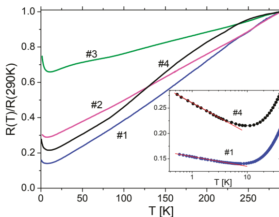
Figure 8. The temperature dependencies of the out-of-plane resistance R_{\perp}(T) for crystals 1–4 . The R(290\text{K}) values are 287 Ohm, 3.77 kOhm, 2.52 kOhm, and 427 Ohm, respectively. The inset shows the resistance R(T)/R(290\text{K}) as function of T in the logarithmic scale for the samples 1 and 4 .
