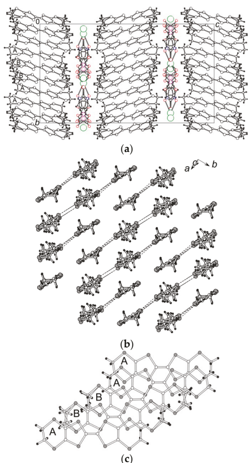
Figure 2. (a) Projection of the structure of 4 along a (the minor part of the [\text{Ga}(\text{ox})_3]^{3-} anion is omitted, except for Ga1B and K2 atoms); (b) view of the radical cation \beta'' -layer along the long axis of BEDT-TTF with short intermolecular S...S contacts < 3.6 \text{ \AA} (dashed lines); and (c) overlap modes within the stack.
